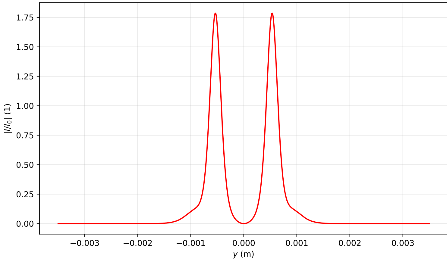
Intensity profile I(x=0, y, z=0.557)/I_0 , P_{in}=8.0P_{cr} , artificial time
